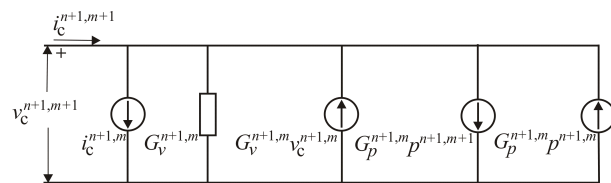
Fig. 1. The linearized and discretized model of the capacitor controlled by pressure
